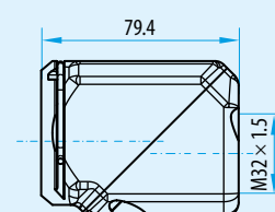
Straight cable exit
