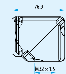
Right-angled cable exit
