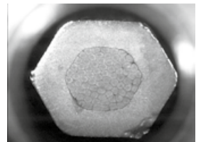
Microsection hexagonal crimping
